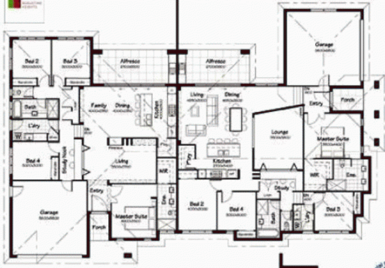
Ground Floor 1:100
