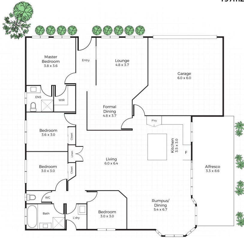
Floor Plan Ground Floor
