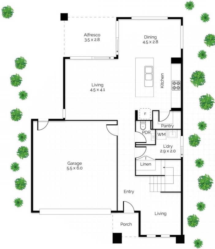
Floor Plan Ground Floor
