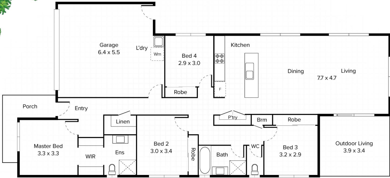
Floor Plan Ground Floor
